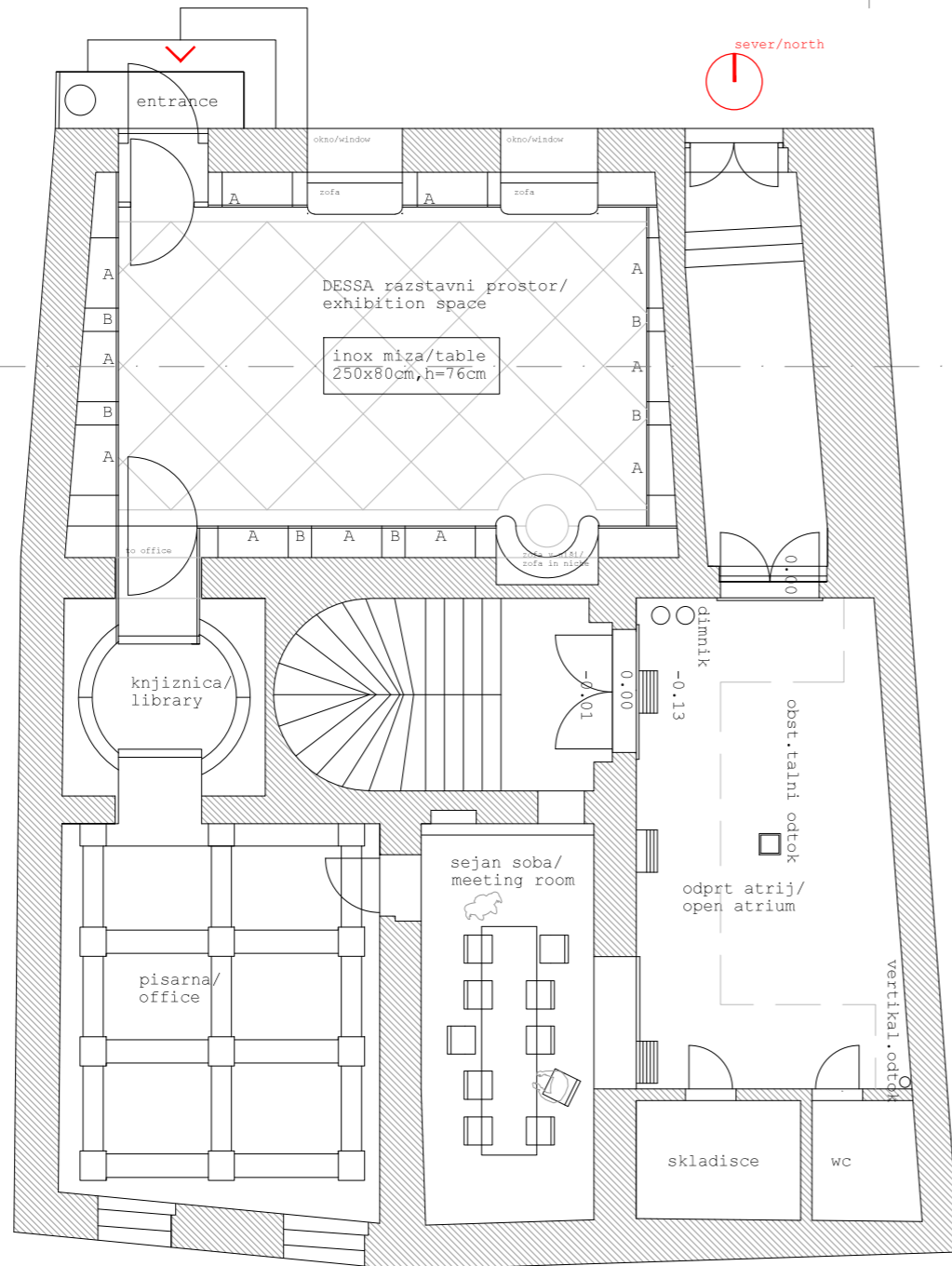
TLORIS/PLAN VIEW
